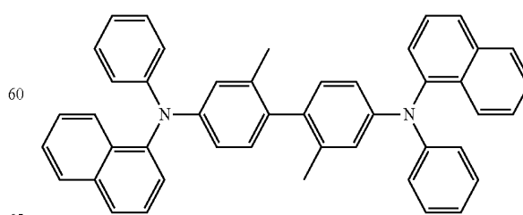
methylated NPB
